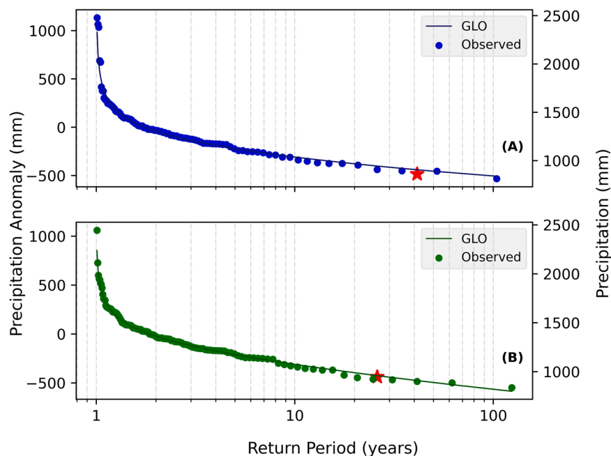
Fig. 4. Return period for both stations in the univariate framework. (A) Piracicaba (B) Campinas. The annual observed precipitation, concerning the 2014–2015 drought in the study region, is shown in red. (For interpretation of the references to color in this figure legend, the reader is referred to the web version of this article.)
