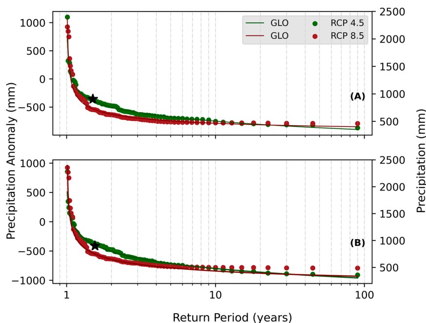
Fig. 7. Return period for both stations in the univariate framework considering future scenarios. (A) Piracicaba and (B) Campinas. The annual observed precipitation concerning the 2014–2015 drought in the study region, is shown in black. Anomalies were computed considering the mean precipitation of the observed data.
