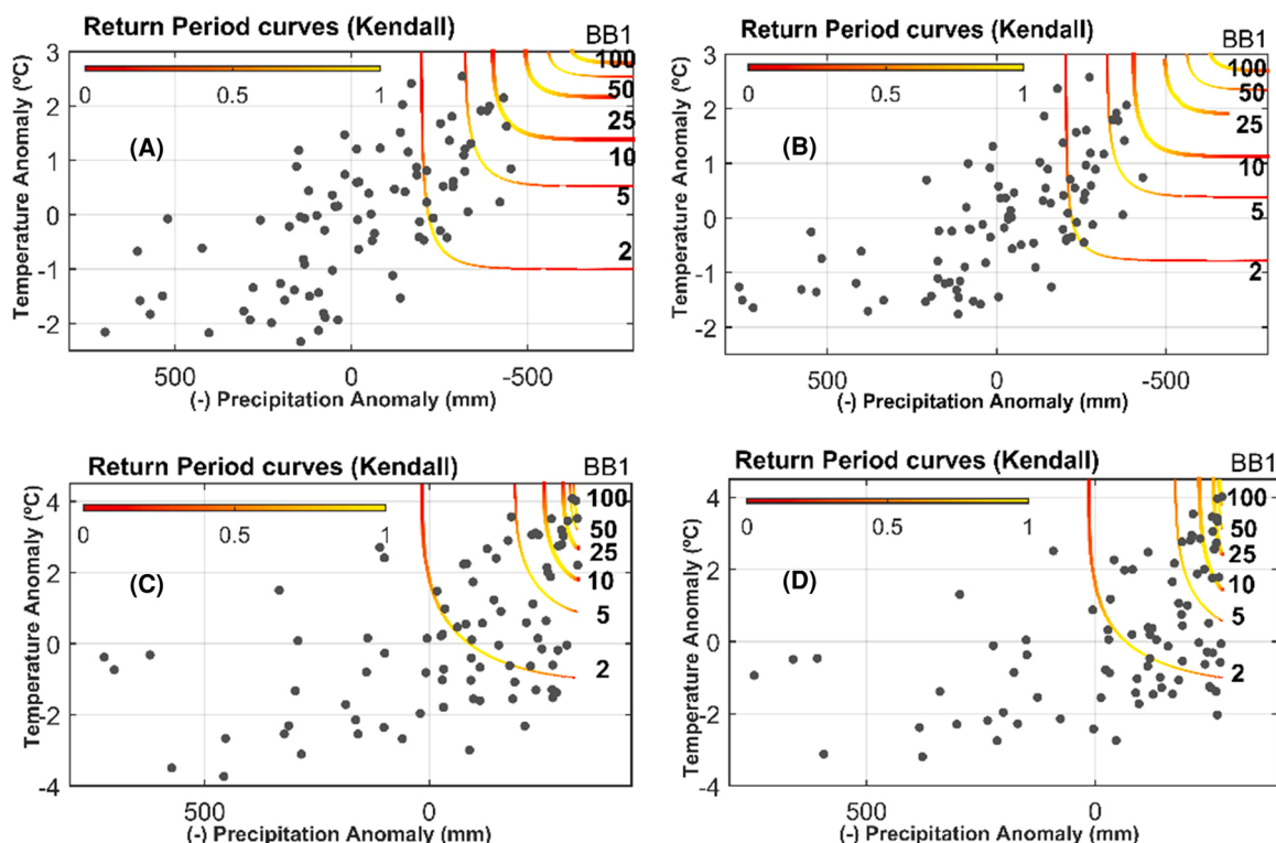
Fig. 8. Joint probability isolines associated with 2, 5, 10, 25, 50, and a 100-year return period for Campinas considering RCP4.5 (A) and RCP8.5 (C) scenarios. The same for Piracicaba, where RCP4.5 and RCP8.5 are represented in (B) and (D), respectively. Isolines are colored with joint density levels, in which yellow and red represent the highest and lowest levels, respectively. The most likely quantile is associated with the highest density level. Isolines are calculated for “Future Anomalies”. (For interpretation of the references to color in this figure legend, the reader is referred to the web version of this article.)
