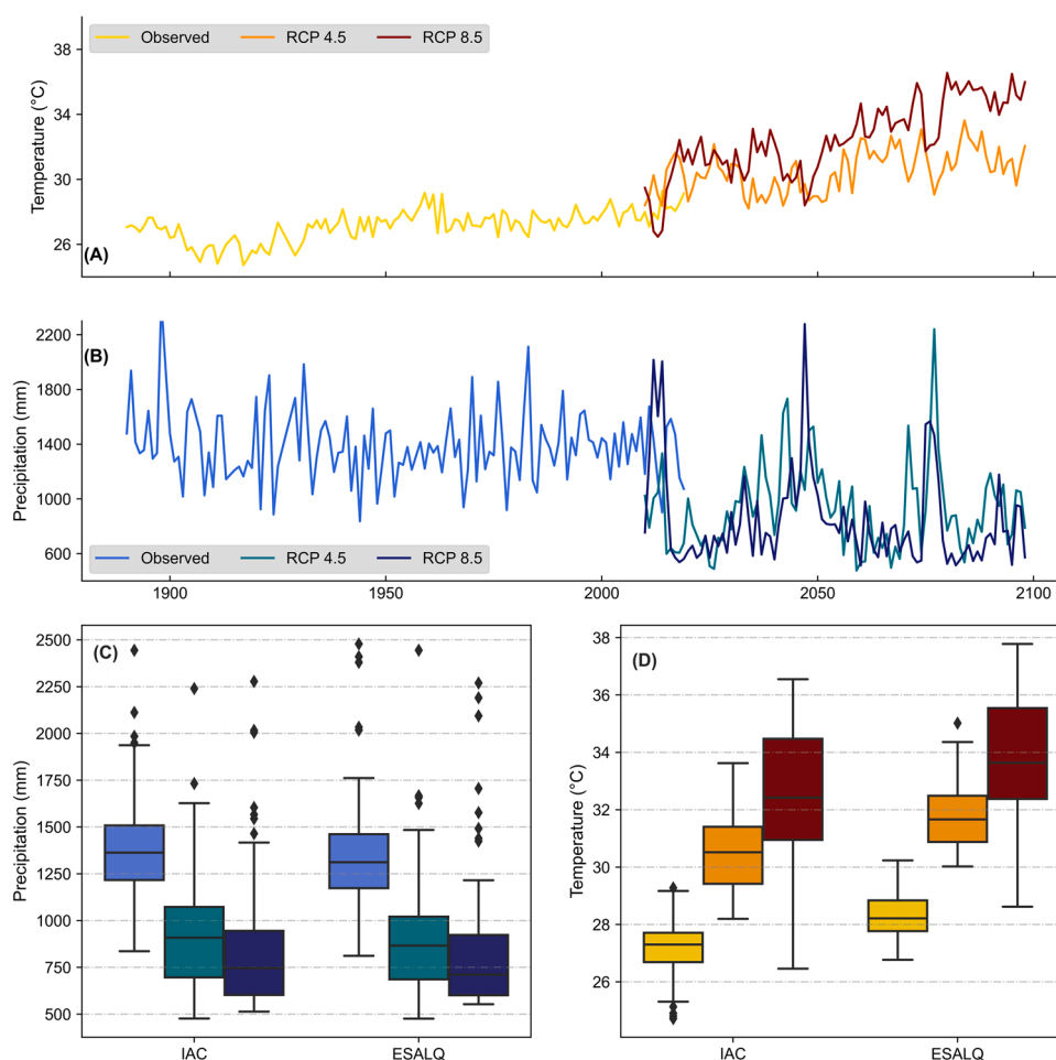
Fig. 3. Temperature (A) and precipitation (B) series of Campinas for the observed period and future scenarios (RCP 4.5 and RCP 8.5). Boxplot showing precipitation (C) and temperature (D) data for Campinas (IAC) and Piracicaba (ESALQ). The colors of the boxes in Figs. C and D share the same legend as Figs. A and B. (For interpretation of the references to color in this figure legend, the reader is referred to the web version of this article.)
