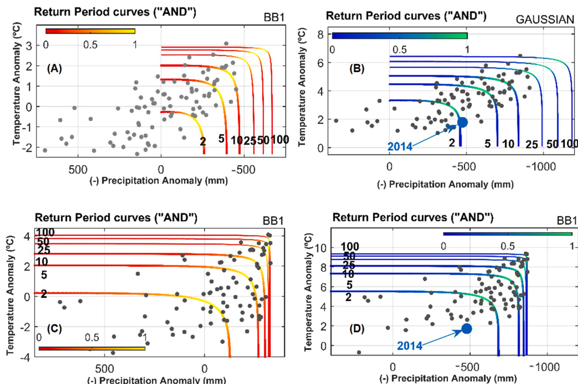
Fig. 10. Joint probability isolines associated with 2, 5, 10, 25, 50 and 100-year return period for Campinas considering RCP4.5 (top) and RCP8.5 (bottom) scenarios. Isolines were colored according to their level of joint density. Yellow and light blue represent the highest levels, while red and blue represent the lowest levels. The most likely quantile is associated with the highest density levels. Isolines were calculated for both “Future Anomalies” (left) and “Present Anomalies” (right). (For interpretation of the references to color in this figure legend, the reader is referred to the web version of this article.)
